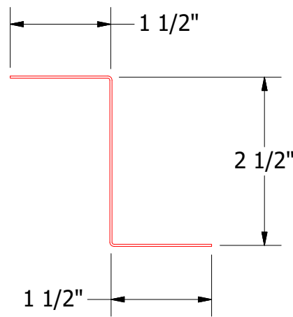
FLA910-Z Closure
