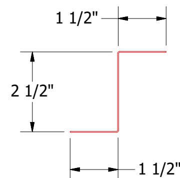
FLA910-Z Closure
