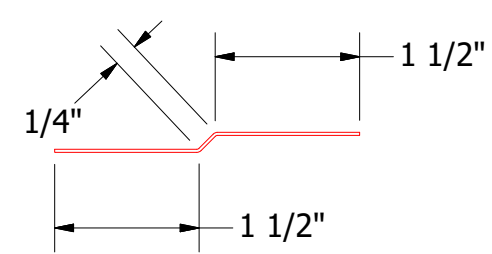
FLA976-Joggle Cleat (NTS)
