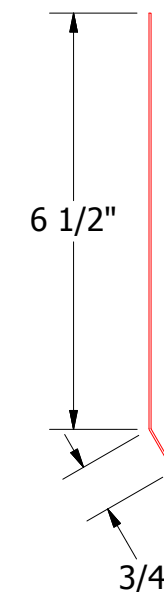
FLA349-Shed Ridge Starter Cleat
