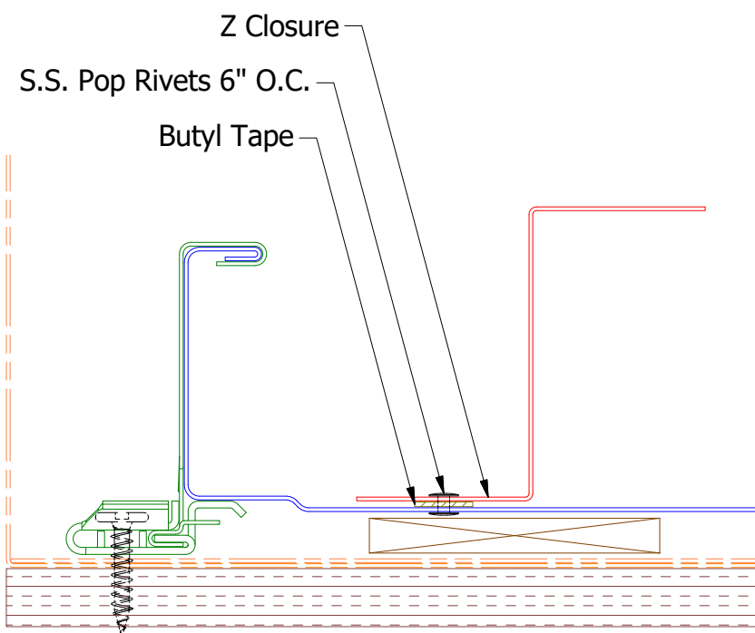
Butyl Tape Detail
