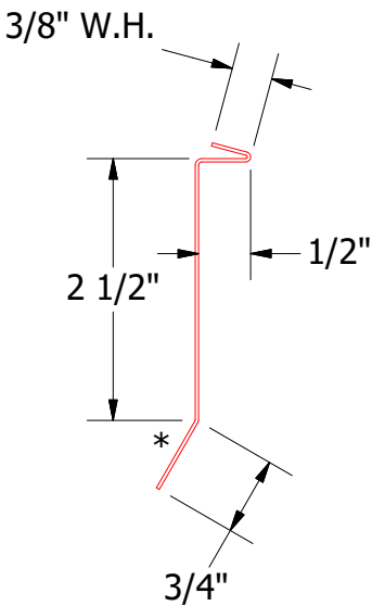
FLA980-Counterflashing
