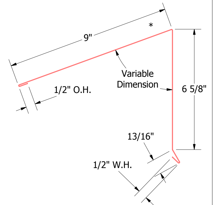
FLA346-Shed Ridge Cap
