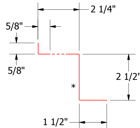
FLA911-Vented Z Closure
