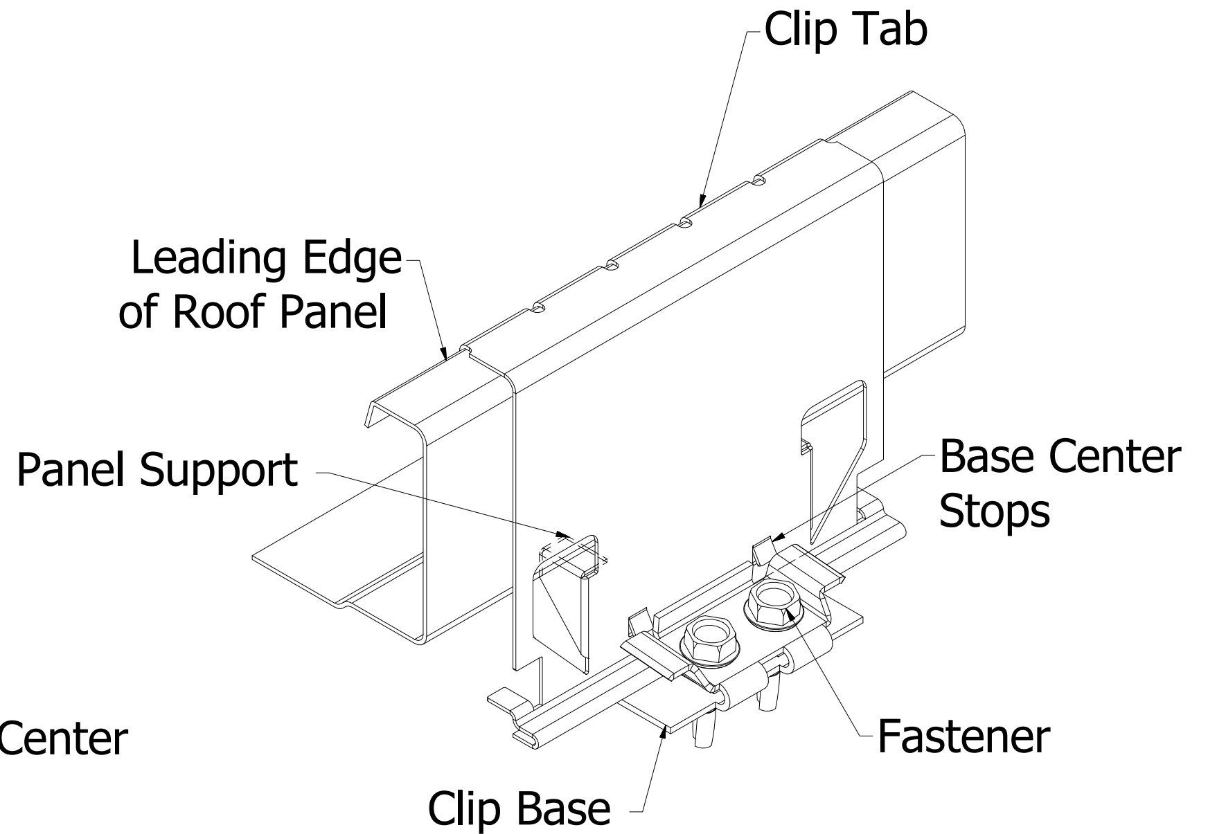
1 3/8" Stand-Off Clip
