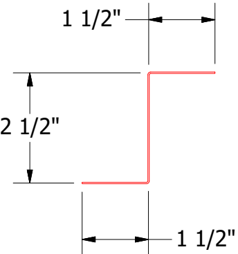
FLA910-Z Closure
