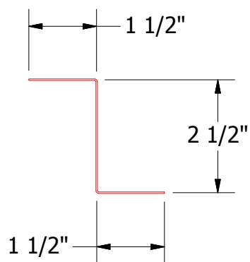
FLA910-Z Closure
