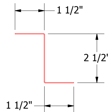
FLA910-Z Closure
