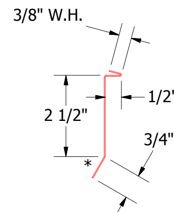
FLA980-Counterflashing
