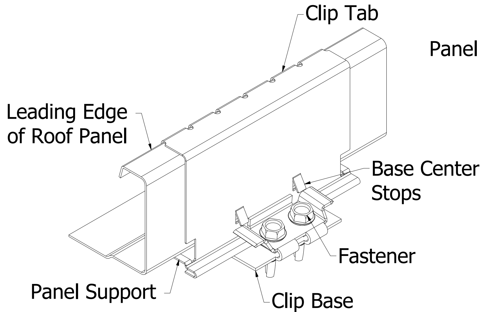
3/8" Stand-Off Clip
