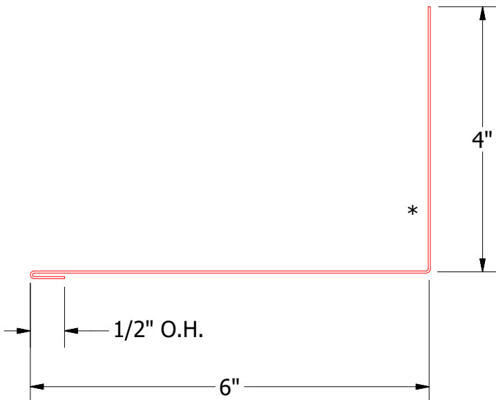
FLA411-Sidewall Trim
