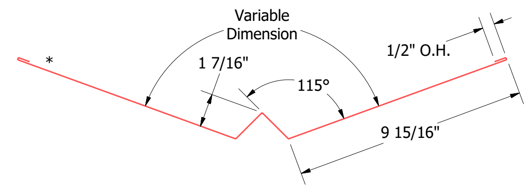
FLA800-Valley Trim
