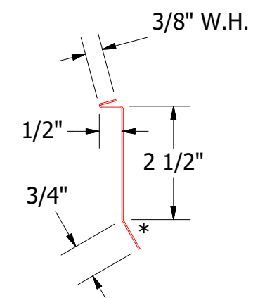
FLA980-Counterflashing
