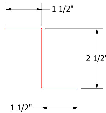
FLA910-Z Closure
