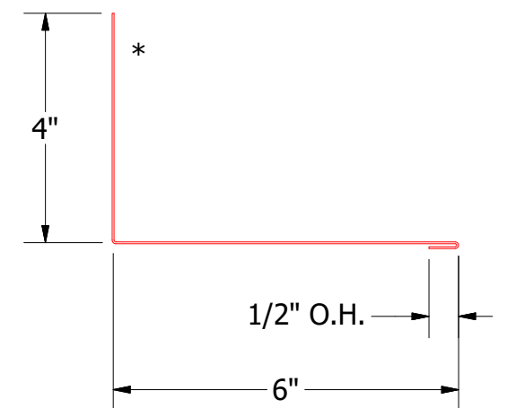
FLA411-Sidewall Trim
