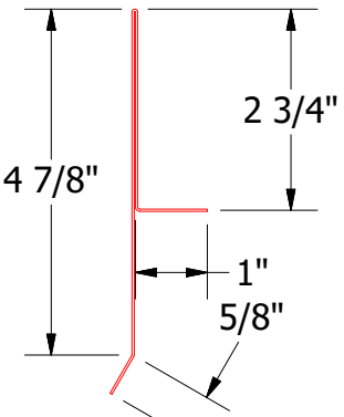
FLA211-Gable Starter Cleat
