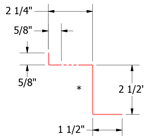
FLA911-Vented Z Closure
