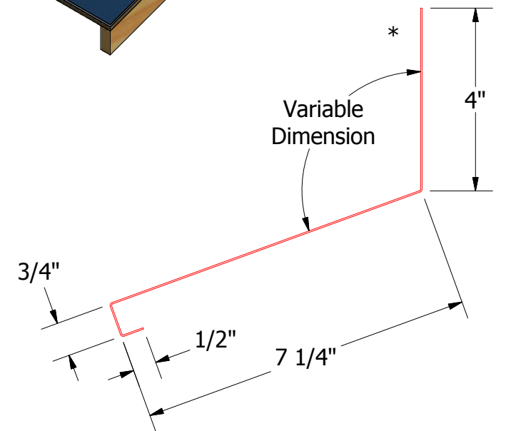
FLA510-Vented Headwall Trim
