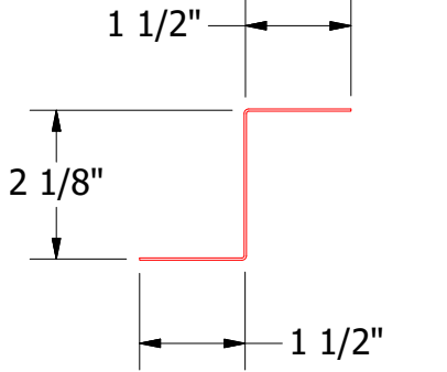
FLA912-Z Closure
