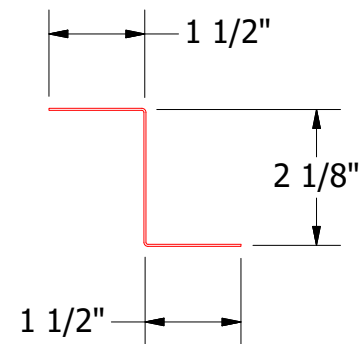
FLA912-Z Closure
