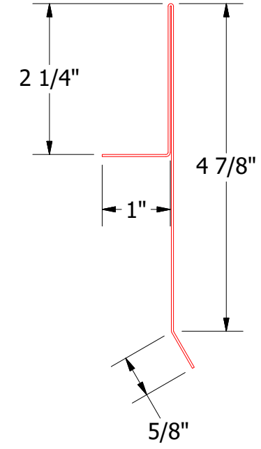
FLA215-Gable Starter Cleat
