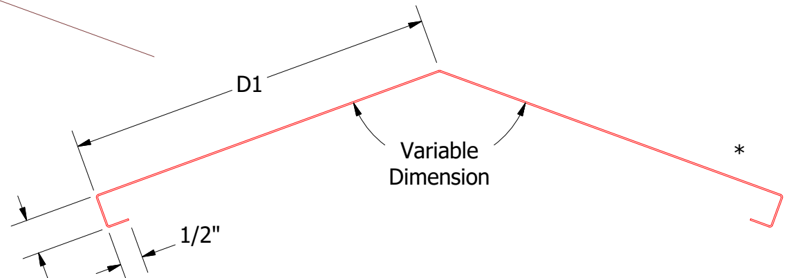
Vented Ridge Cap
