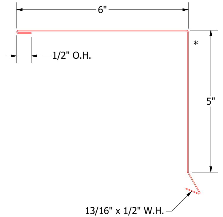
FLA210-Gable Trim Cap
