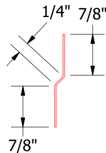
FLA975-Joggle Cleat
