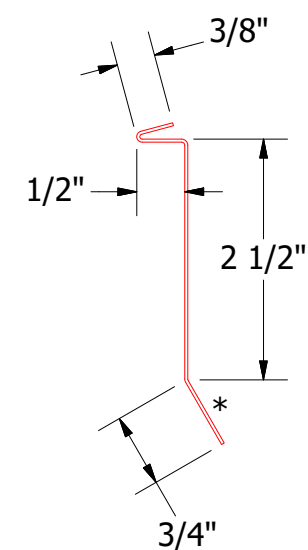
FLA980-Counterflashing
