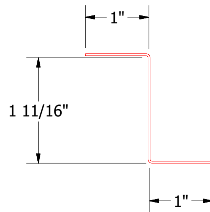
FLA916-Z Closure
