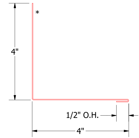
FLA410-Sidewall Trim
