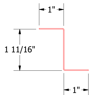
FLA916-Z Closure
