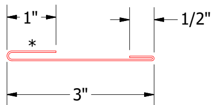
FLA962-Utility Cleat
