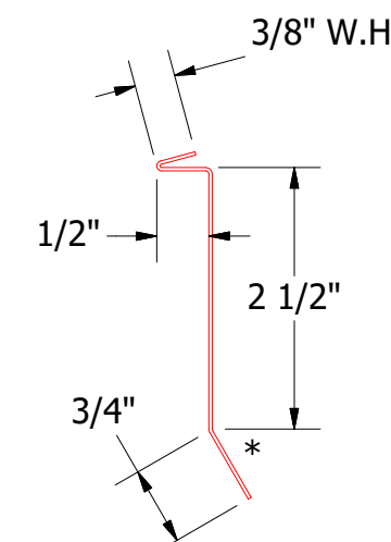
FLA980-Counterflashing
