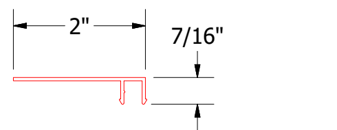
Receiver Extrusion for Jamb Cover
