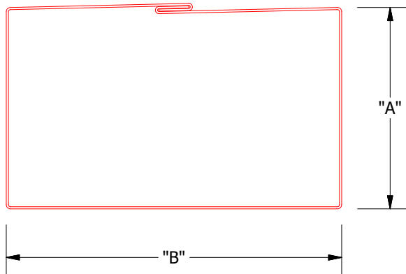
Downspout Offset Interlock
