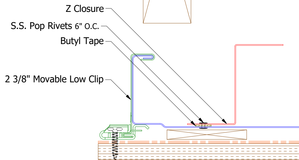
Butyl Tape Detail
