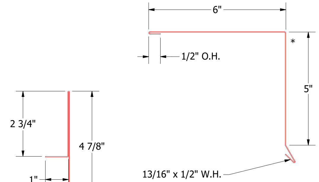
FLA210-Gable Trim
