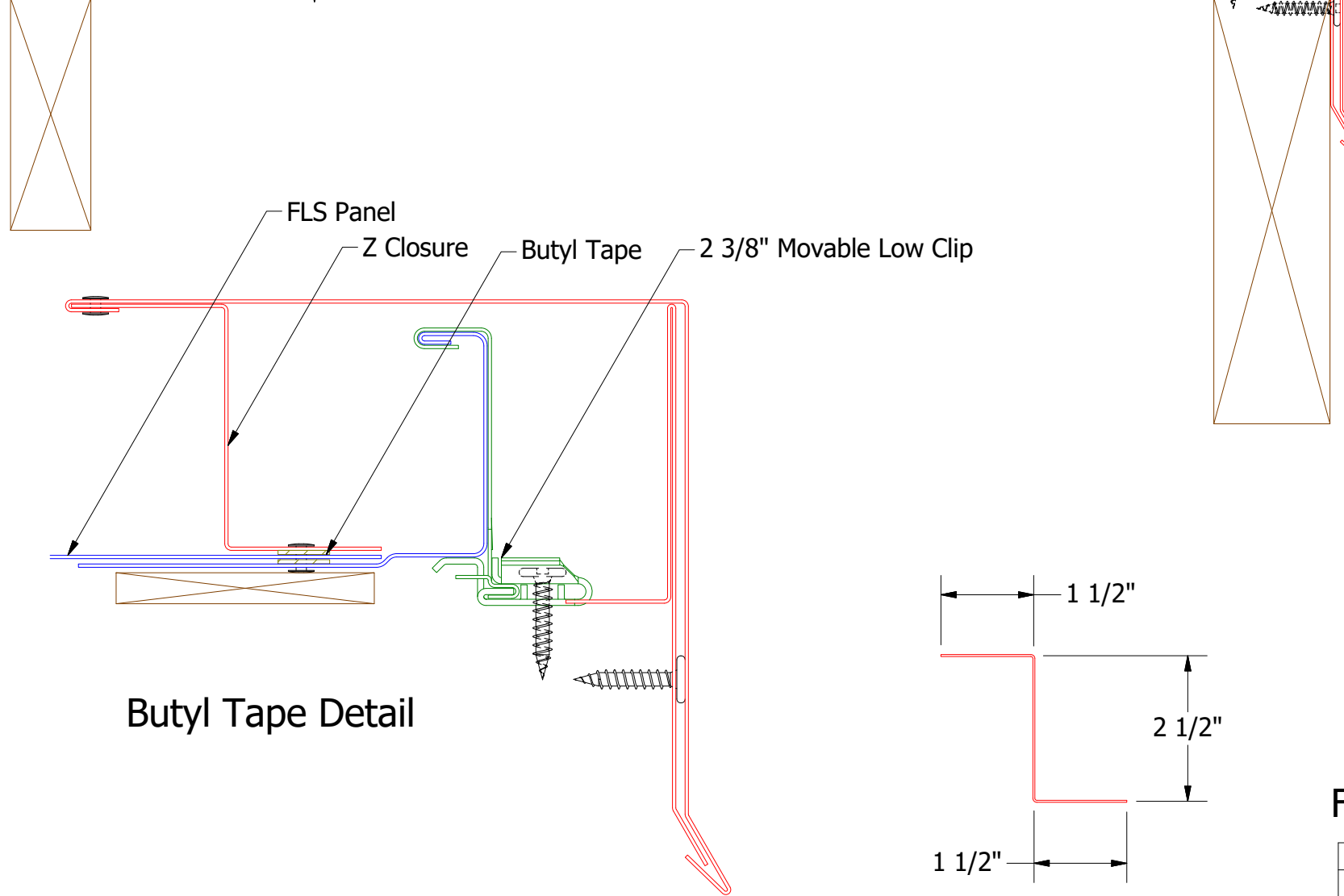
FLA910-Z Closure
