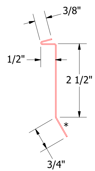
FLA980-Counterflashing
