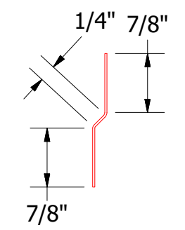
FLA975-Joggle Cleat
