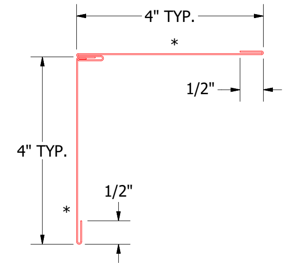
SFC999-Curved Gable Trim
