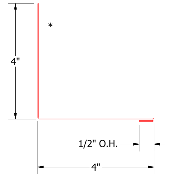
FLA410-Sidewall Trim
