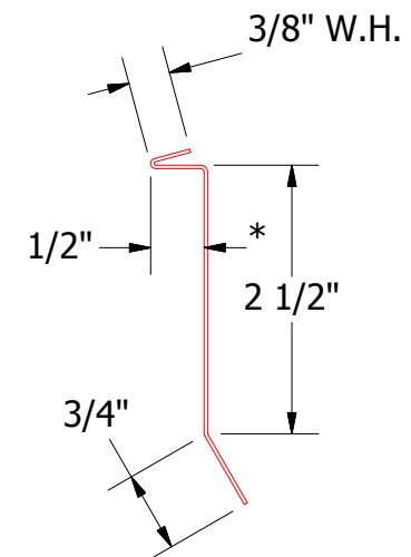
FLA980-Counterflashing
