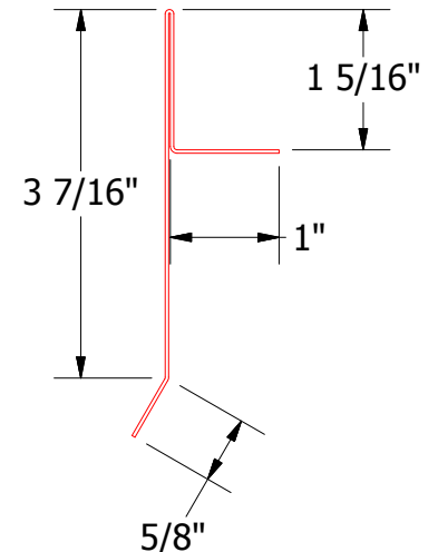
FLA216-Gable Starter Cleat
