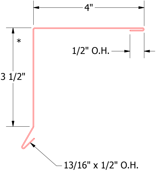
FLA212-Gable Trim Cap
