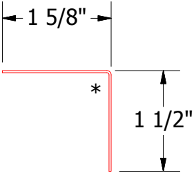
BWA680 - Angle Trim
