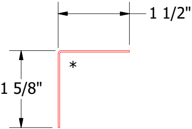
BWA680 - Angle Trim
