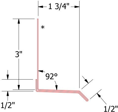
BWA661 - Base Trim
