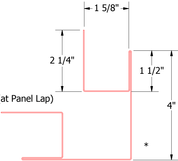
BWA602 - Outside Corner Post
