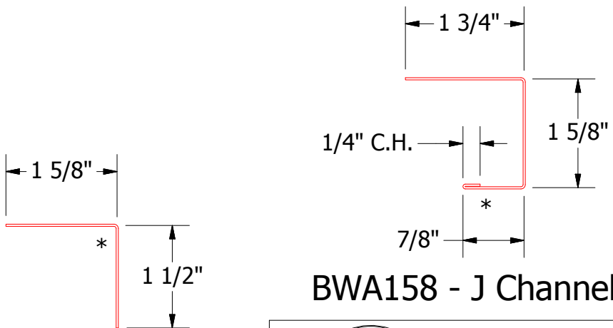
BWA680 - Ange Trim
