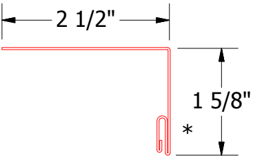
BWA159 - Snap J Base
