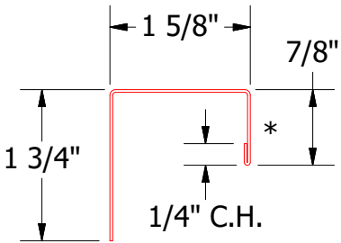
BWA158 - J Channel
