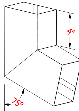
Right Elbow
