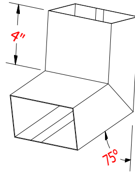
Out Elbow
