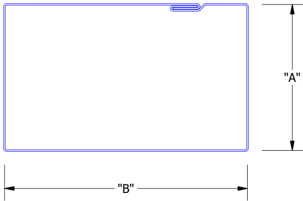
Downspout Interlock
