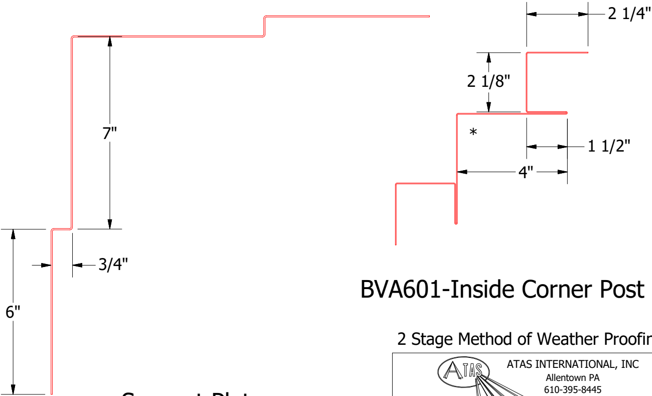
Support Plate
