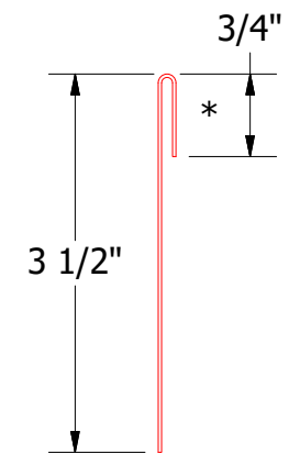
VSA962-Utility Cleat without Return
