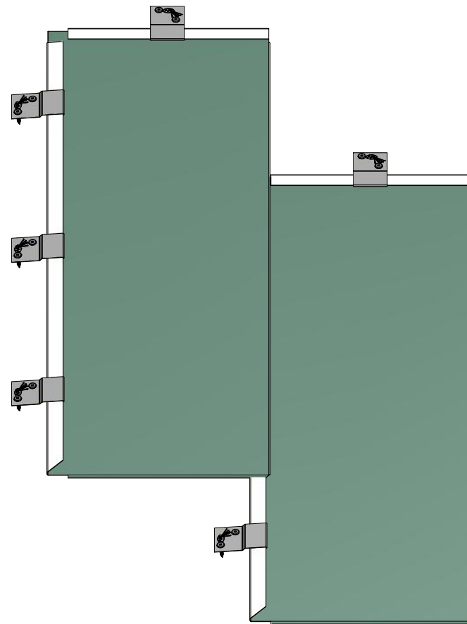
Vertical Installation
