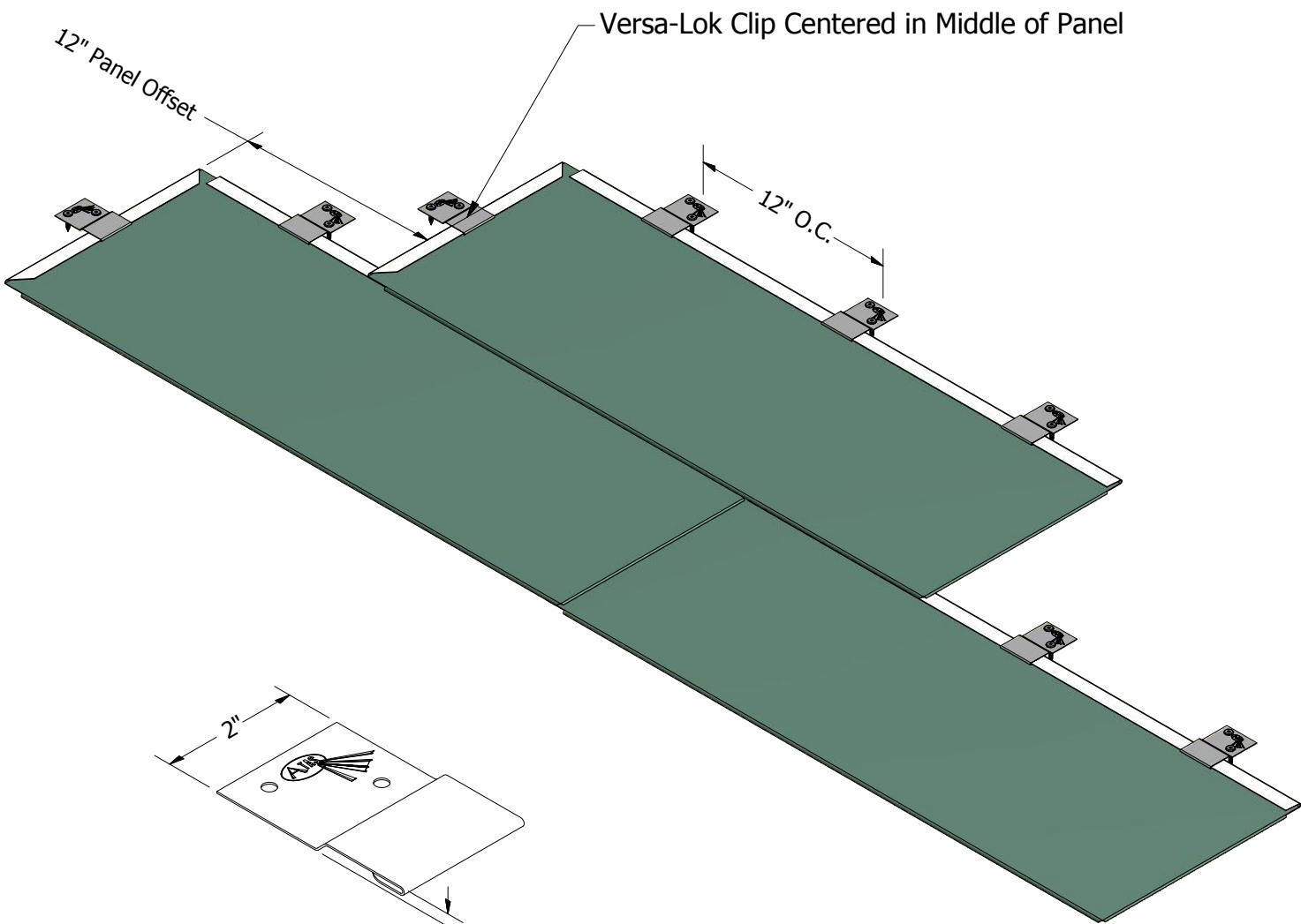
Horizontal Installation
