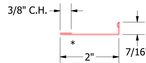
UNS200 - Snap J Cover
