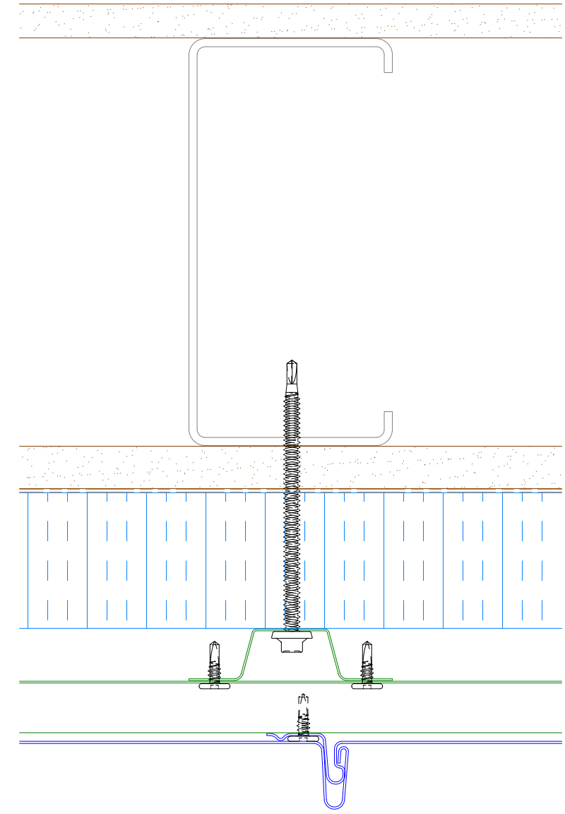
Alternate Subgirt Orientation
