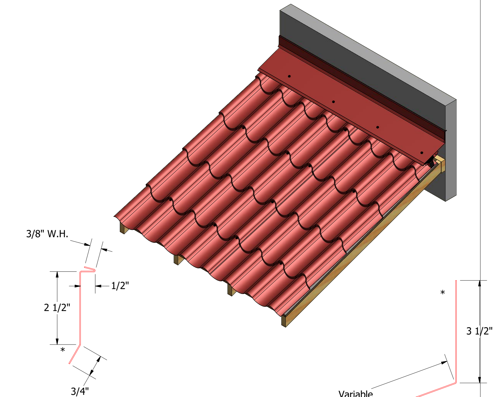
SCA980-Counterflashing
