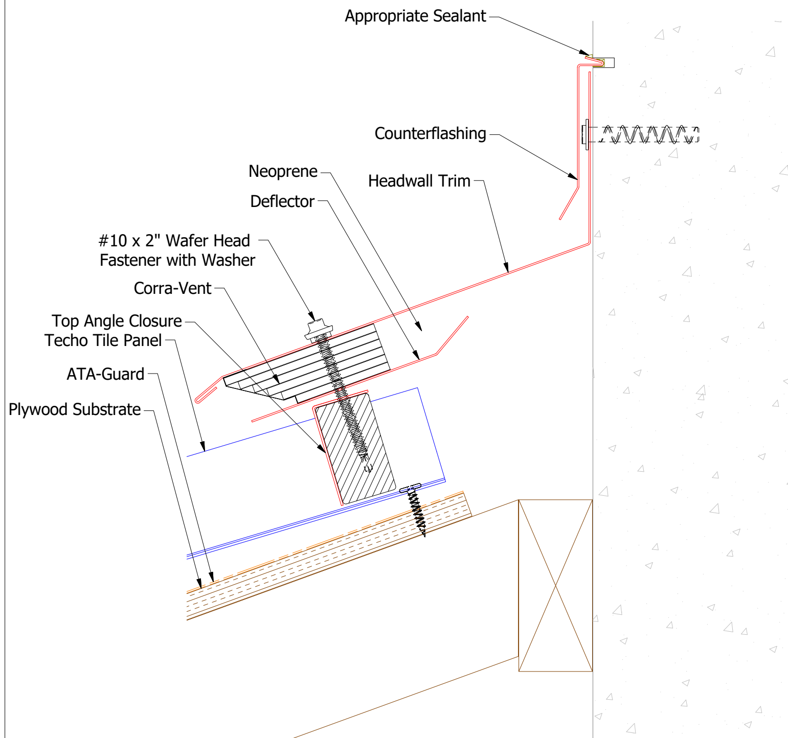
SCA980-Counterflashing
