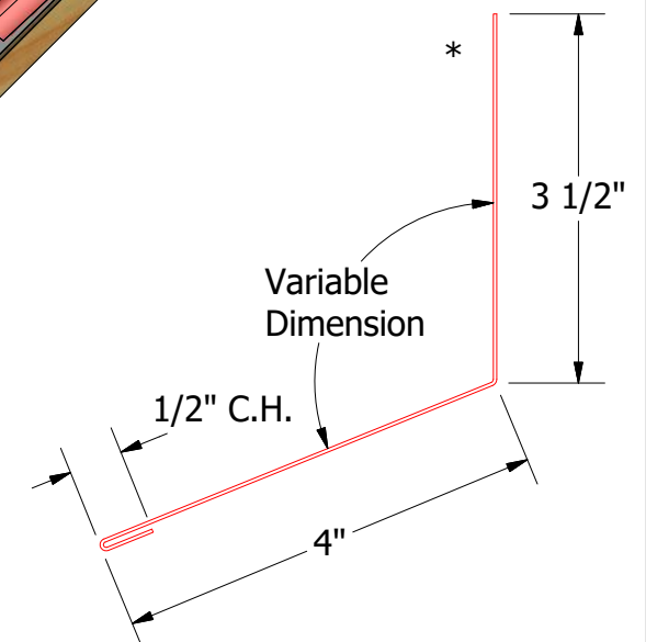
SCA500-Headwall Trim
