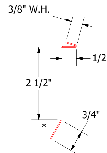
SCA980-Counterflashing
