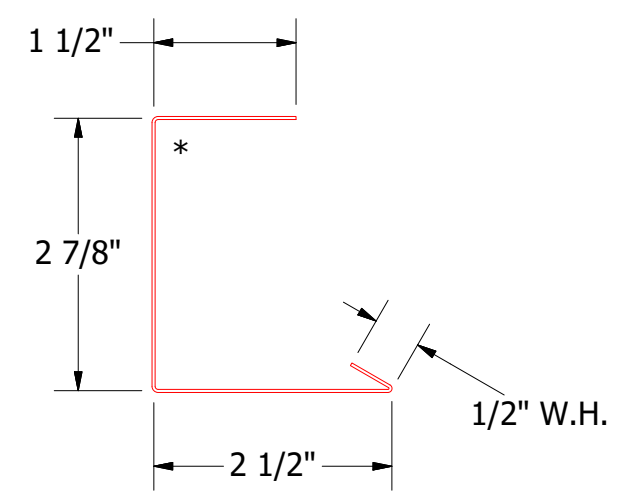
SCA270-Channel Trim
