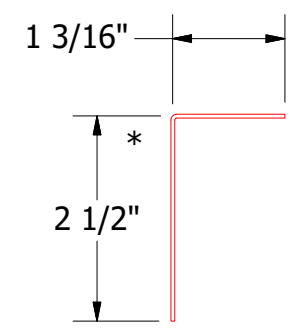
SCA710-Top Closure Angle
