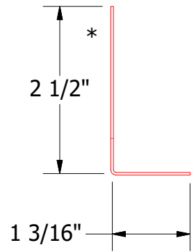
Vented Bottom Closure Angle
