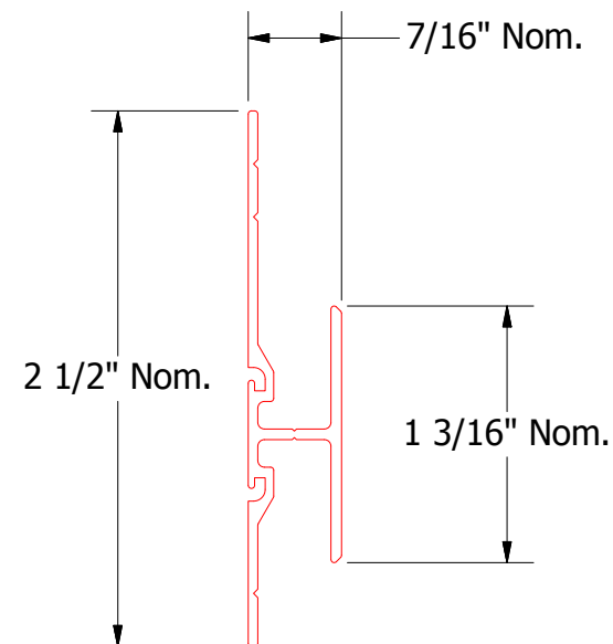
H Molding Extrusion
