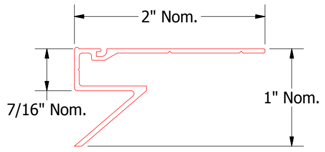
Inside Corner Extrusion
