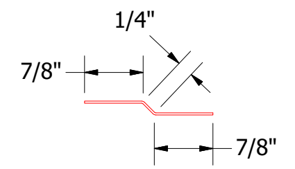
HSA975-Joggle Cleat
