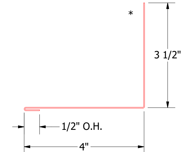
HSA410-Sidewall Trim
