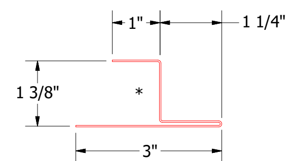
HSA930-Pocket Z Closure (Standard)
