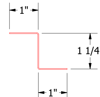
HSA910-Z Closure (Optional)
