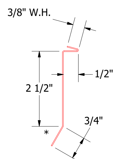
HSA980-Counterflashing
