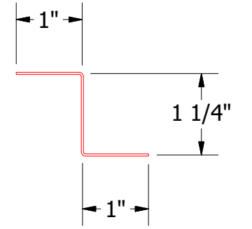
HSA910-Z Closure (Optional)
