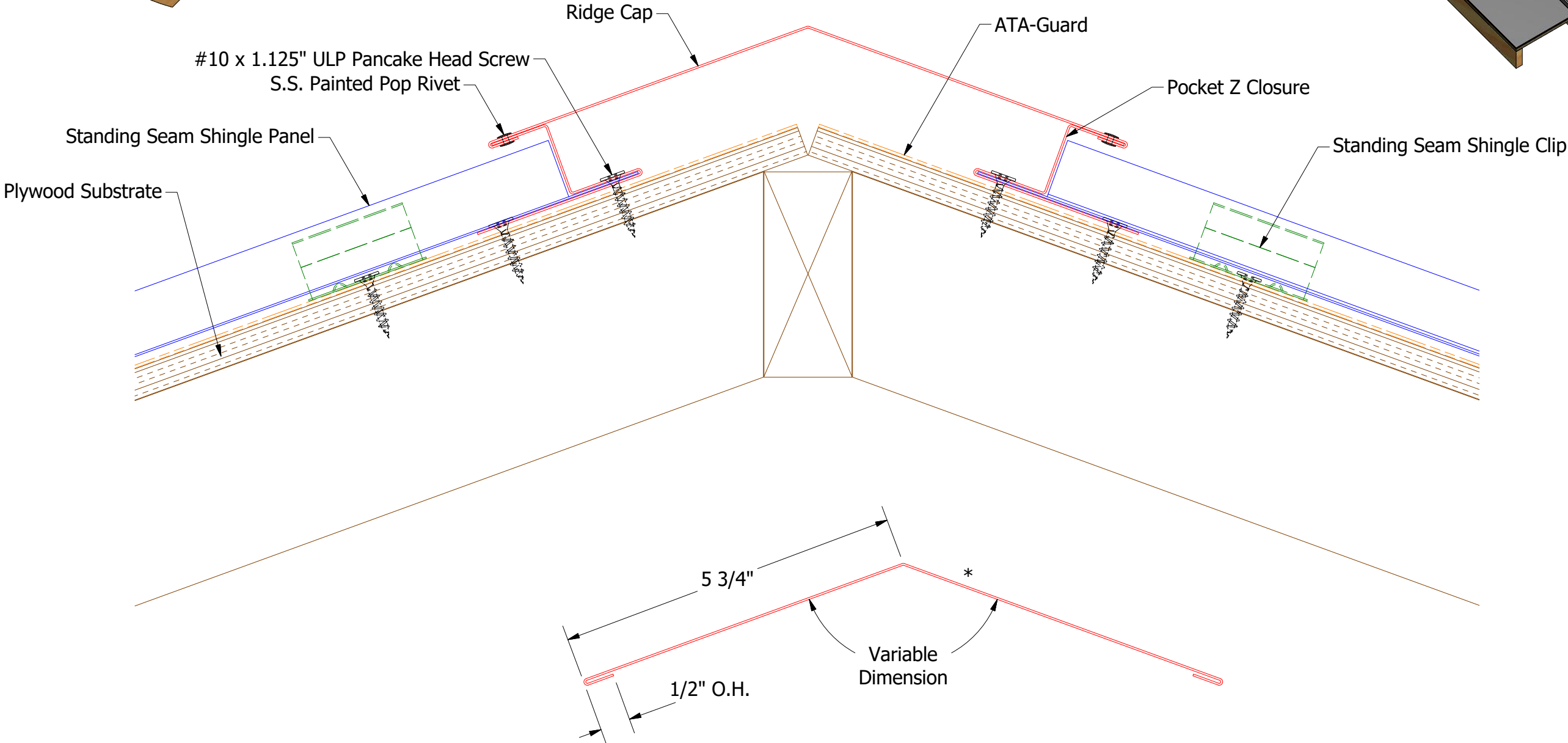
HSA300-Ridge Cap
