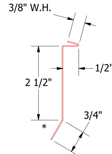
HSA980-Counterflashing
