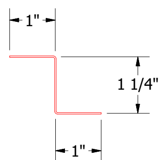
HSA910-Z Closure (Optional)
