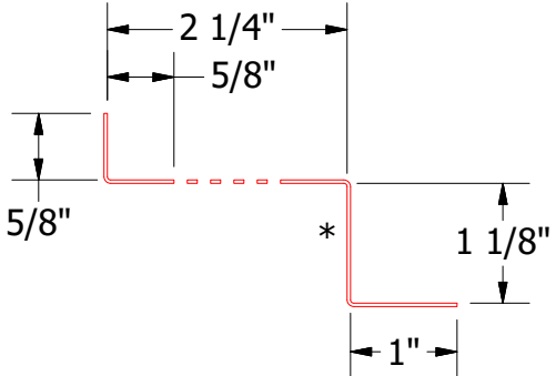
HSA911-Vented Z Closure
