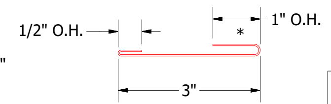
HSA234-Utility Cleat
