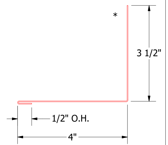
HSA410-Sidewall Trim
