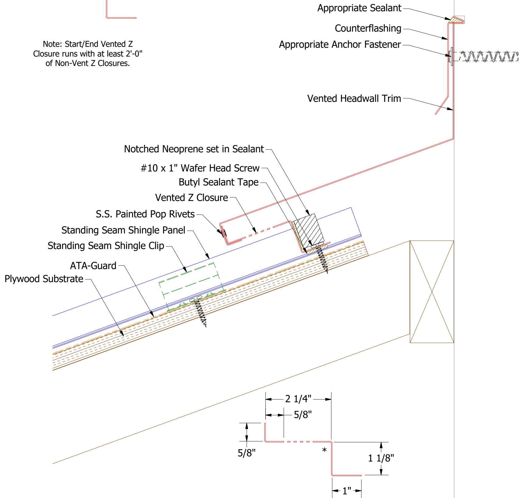
HSA911-Vented Z Closure
