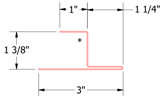
HSA930-Pocket Z Closure (Standard)
