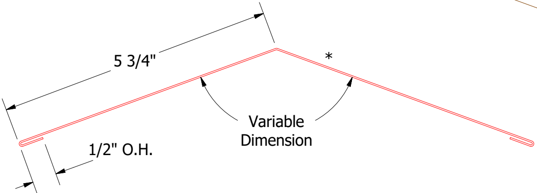
HSA300-Ridge Cap
