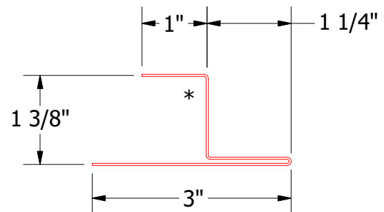
HSA930-Pocket Z Closure (Standard)
