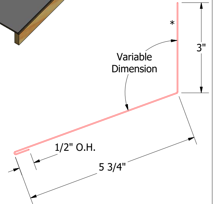
HSA510-Headwall Trim
