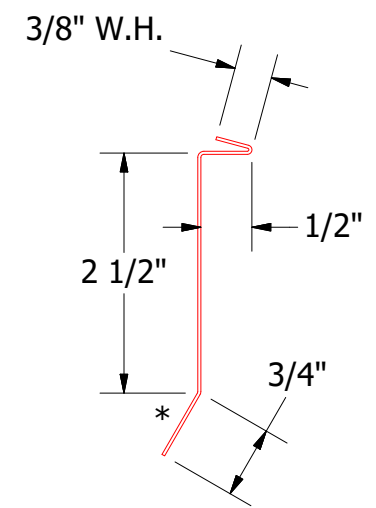
HSA980-Counterflashing
