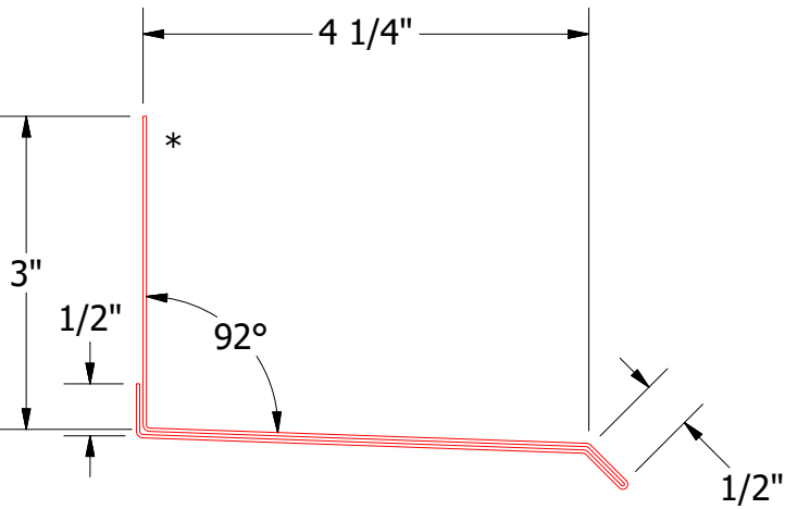
BSA661 - Base Trim
