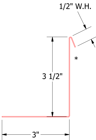
BSA681-Angle Trim with Return
