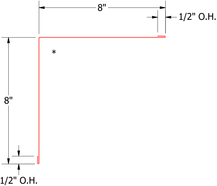
BSA600-Inside Corner Cap
