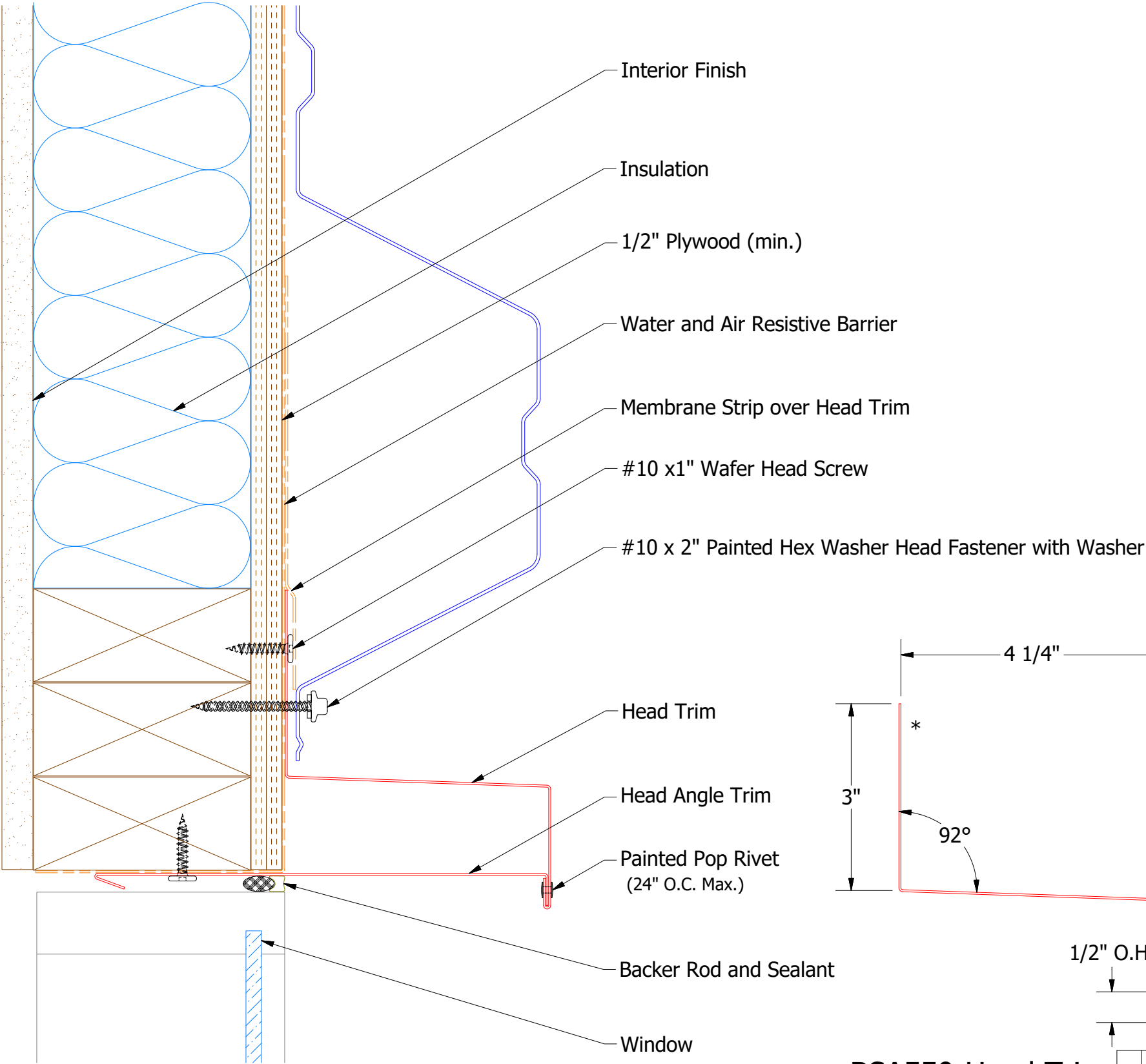
BSA550-Head Trim
