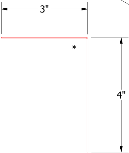
BSA680-Angle Trim
