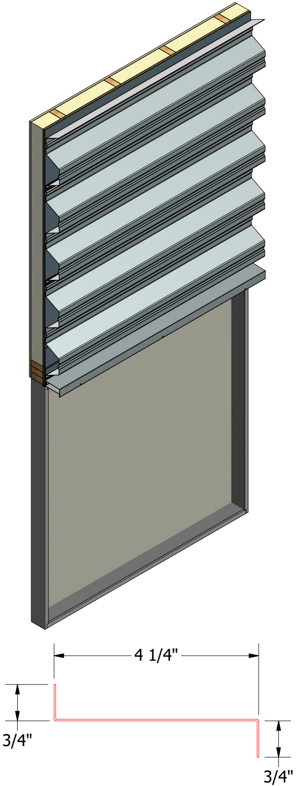
Z Closure
