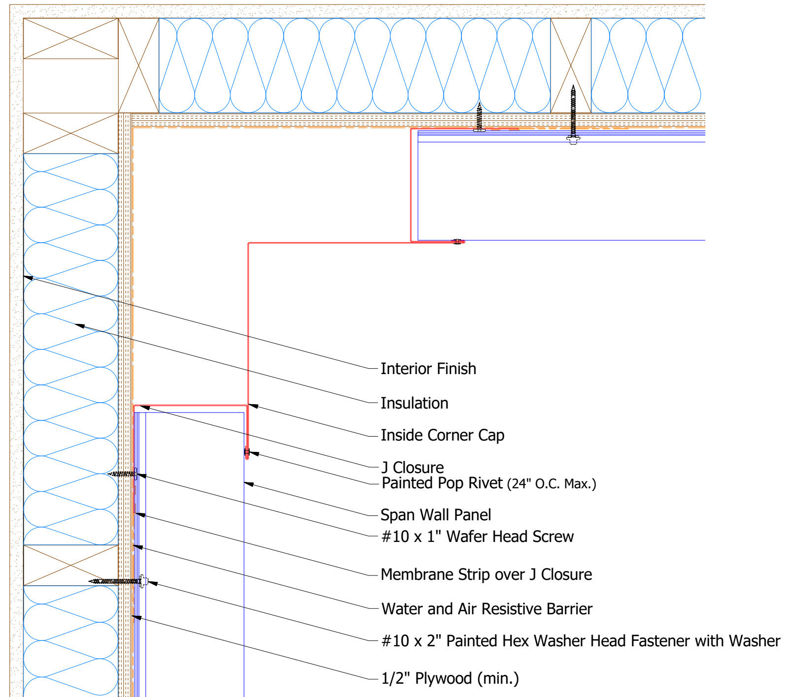
BSA270-J Closure
