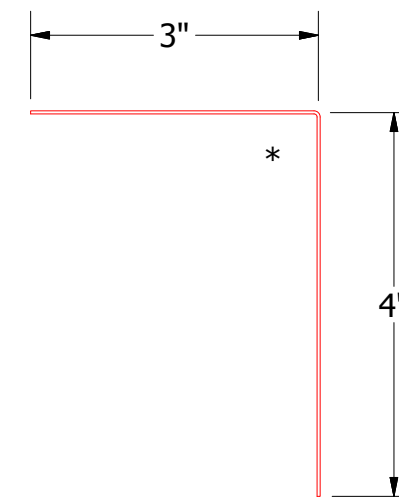
BSA680-Angle Trim
