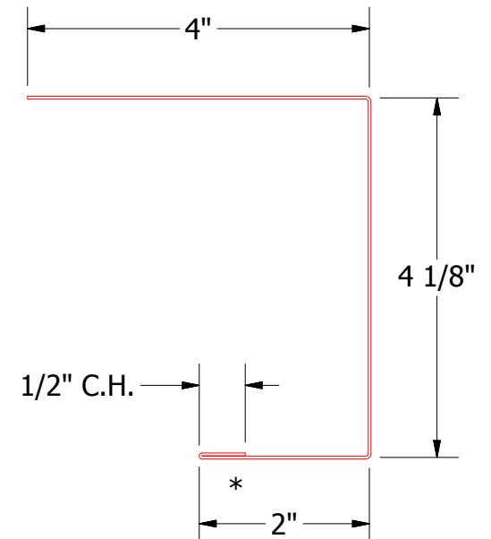
BSA140-J Channel
