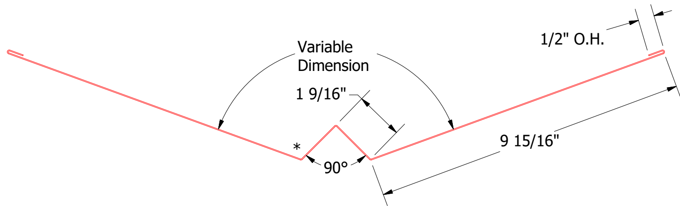
HBA800-Valley Trim
