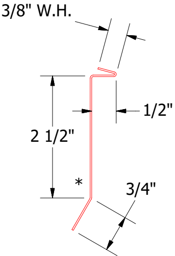
HBA980-Counterflashing
