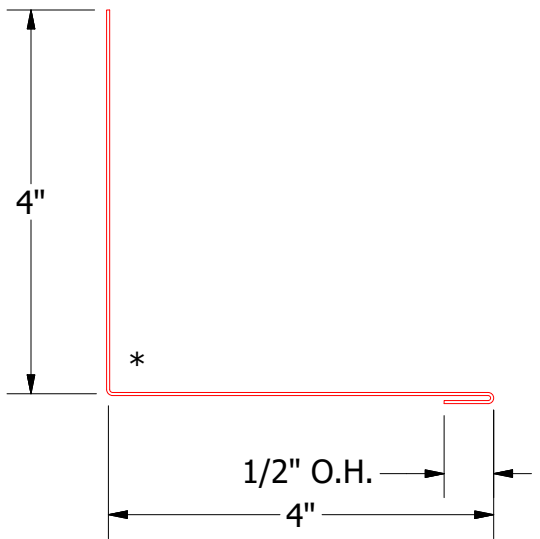
HBA410-Sidewall Trim
