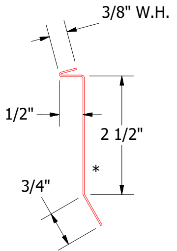
HBA980-Counterflashing
