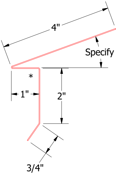
HBA113-Eave Trim
