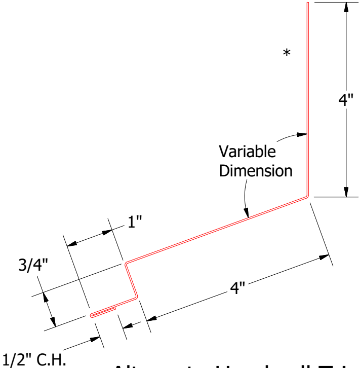
Alternate Headwall Trim
