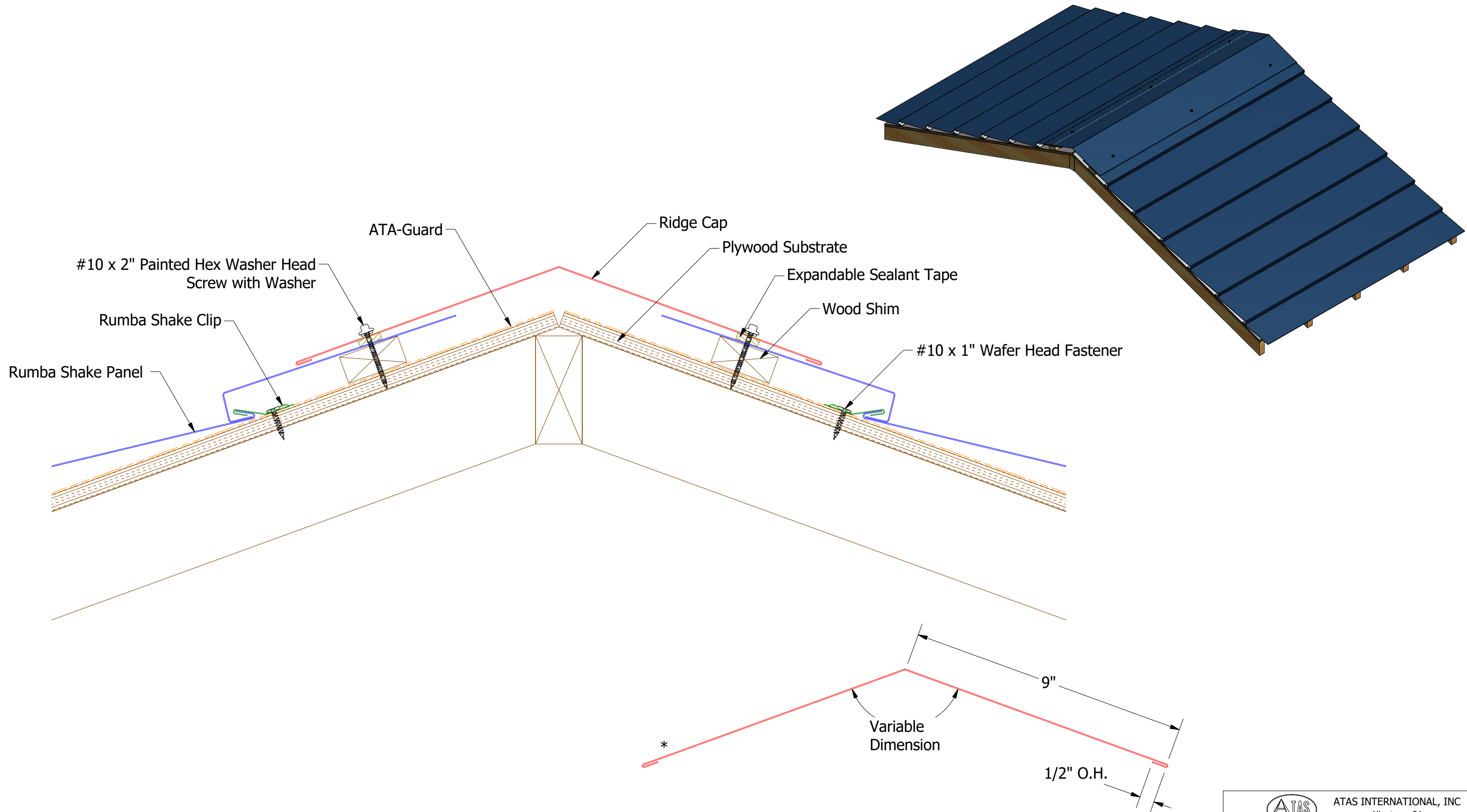
HBA303-Ridge Cap
