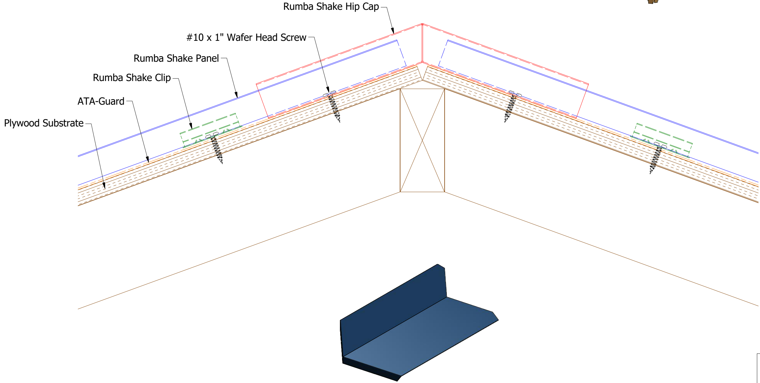
Rumba Shake Hip Cap
