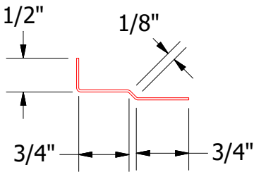
HBA115 - Starter Angle
