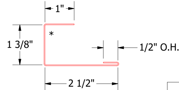
HBA200-Channel Trim
