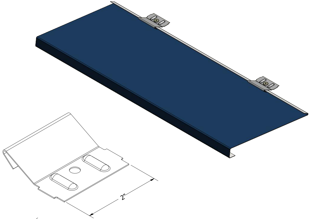
Rumba-Shake Clip HPC906 - 24ga Stainless Steel HPC908 - 24ga Metallic Coated Steel
