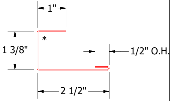
HBA200-Channel Trim
