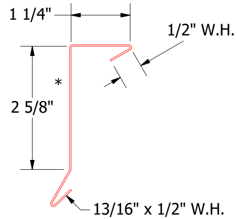
HBA201-Gable Trim Cap
