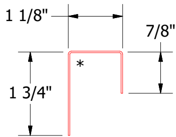
MCA270-J Closure
