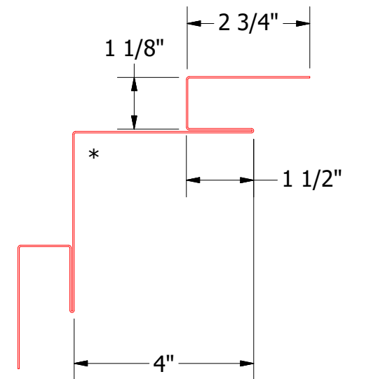
MCA601-Inside Corner Post
