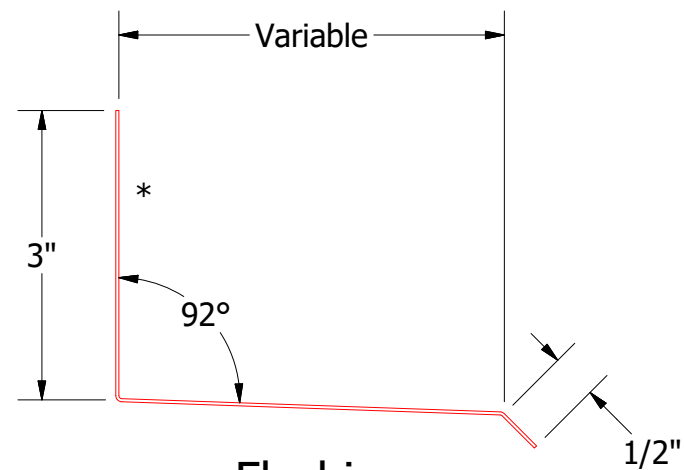
Flashing (Field Fabricated From Color Matched Flat Stock)
