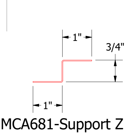
Alternate Subgirt Orientation
