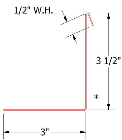
MCA683-Angle Trim with Return
