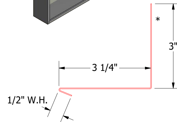
MCA683-Angle Trim with Return
