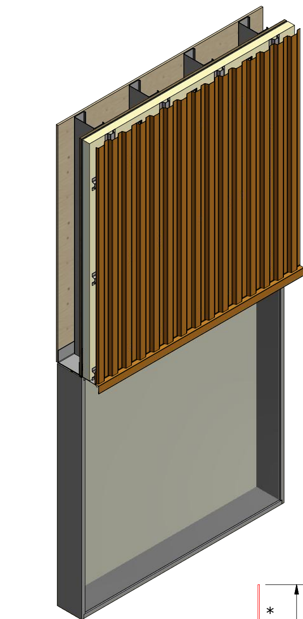
Flashing (Field Fabricated From Color Matched Flat Stock)
