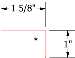
MCA680-Angle Trim
