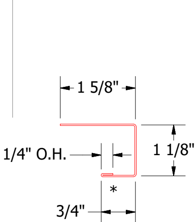
MCA118-J Channel
