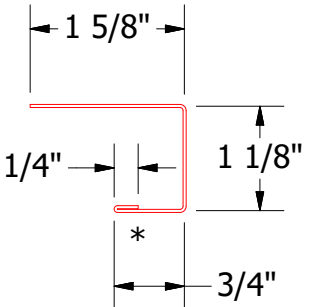
MCA118-J Channel
