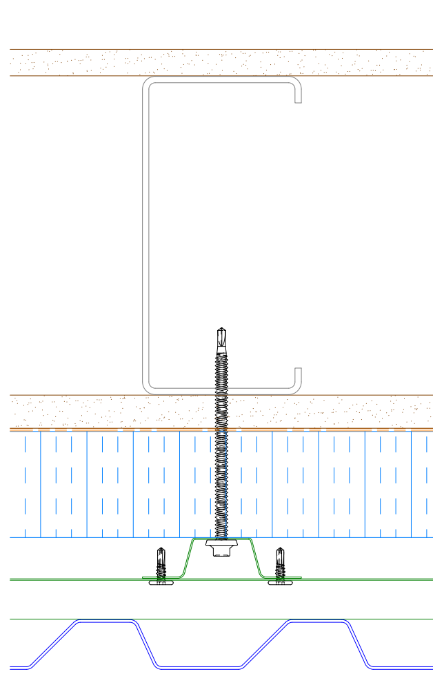
Alternate Subgirt Orientation (NTS)
