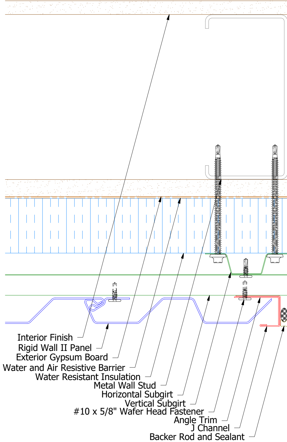
Alternate Subgirt Orientation (NTS)
