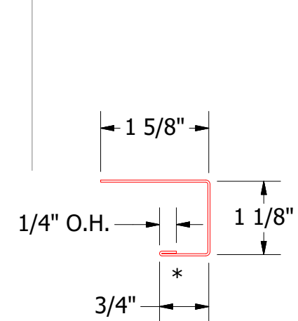
MCA118-J Channel
