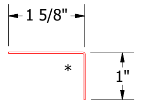
MCA680-Angle Trim
