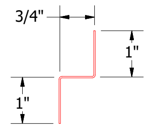
MCA681-Support Z
