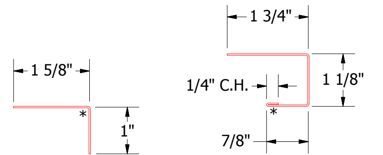
MCA680 - Angle Trim MCA118 - J Channel
