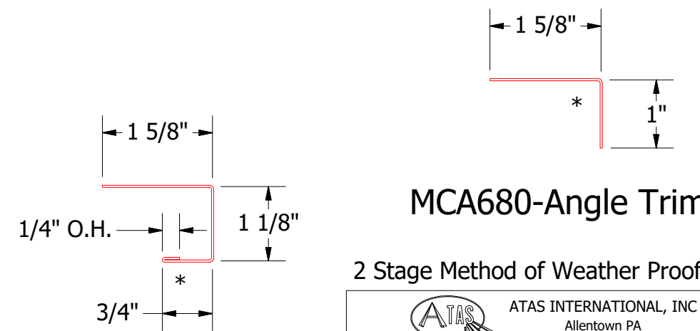
MCA118-J Channel
