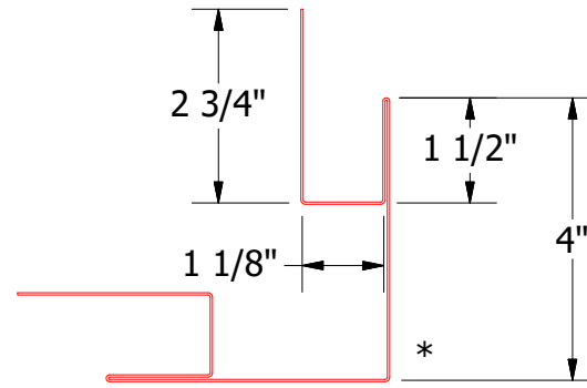
MCA602-Outside Corner Post
