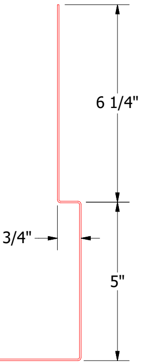
Support Plate
