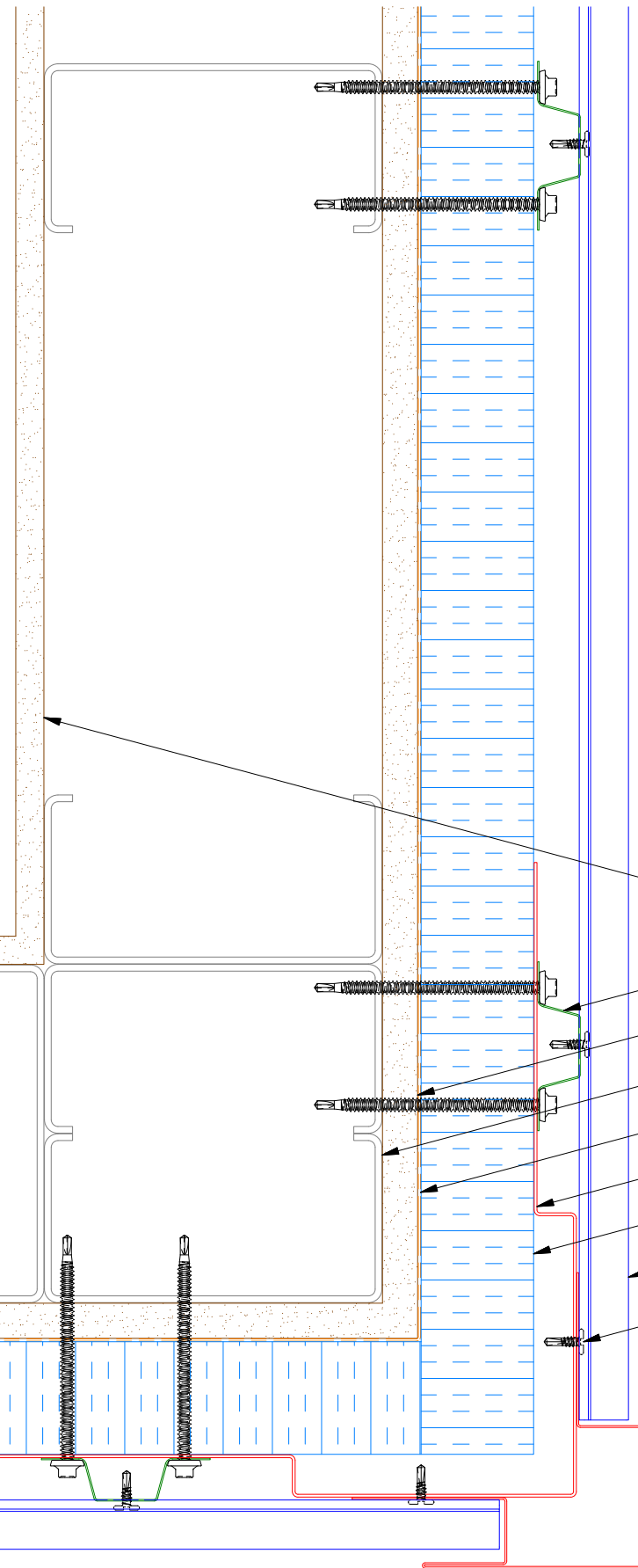
MCA602-Outside Corner Post
