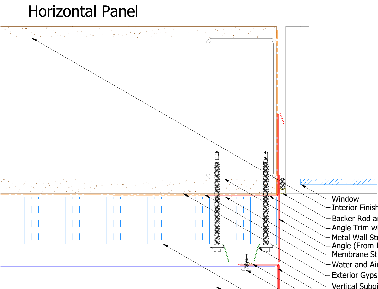
Alternate Subgirt Orientation
