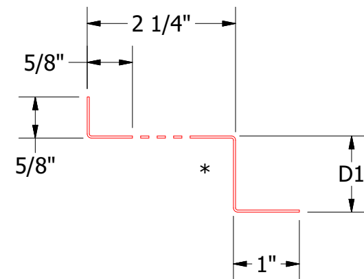
Vented Z Closure PCA911 - 1" Seam and 1" Batten D1=1 1/8" PCA913 - 2" Batten D1=2 1/8"
