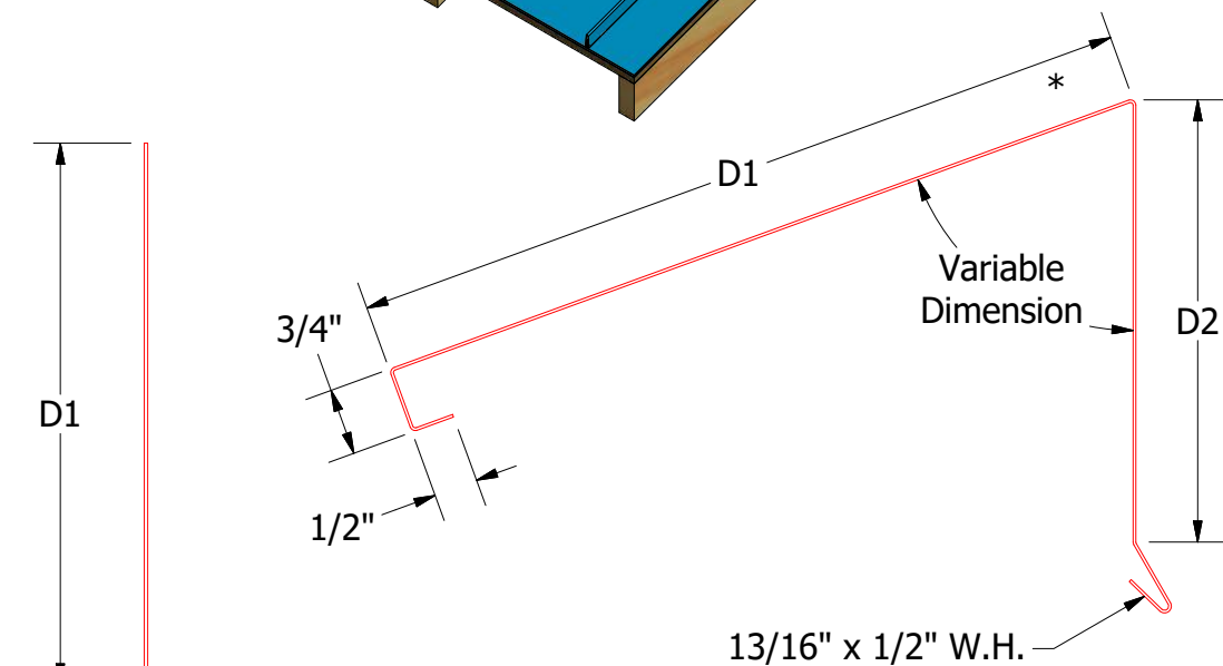
Vented Shed Ridge Cap
