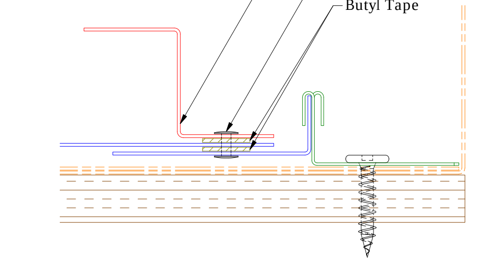
Butyl Tape Detail
