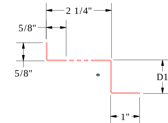
Vented Z Closure PCA911 - 1" Seam and 1" Batten D1=1 1/8" PCA913 - 2" Batten D1=2 1/8"
