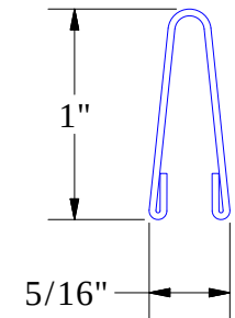
PCS114 - Snap-On PC Seam
