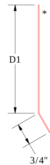
Shed Ridge Starter Cleat
