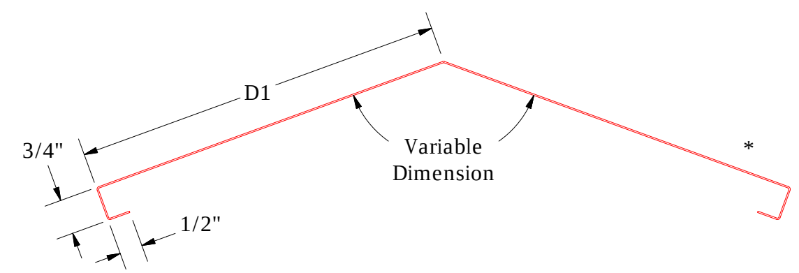
Vented Ridge Cap PCA322-3:12 to 6:12 Slope D1=7 1/4" PCA324-6:12 to 9:12 Slope D1=8 1/4" PCA326-9:12 to 12:12 Slope D1=9 1/4"
