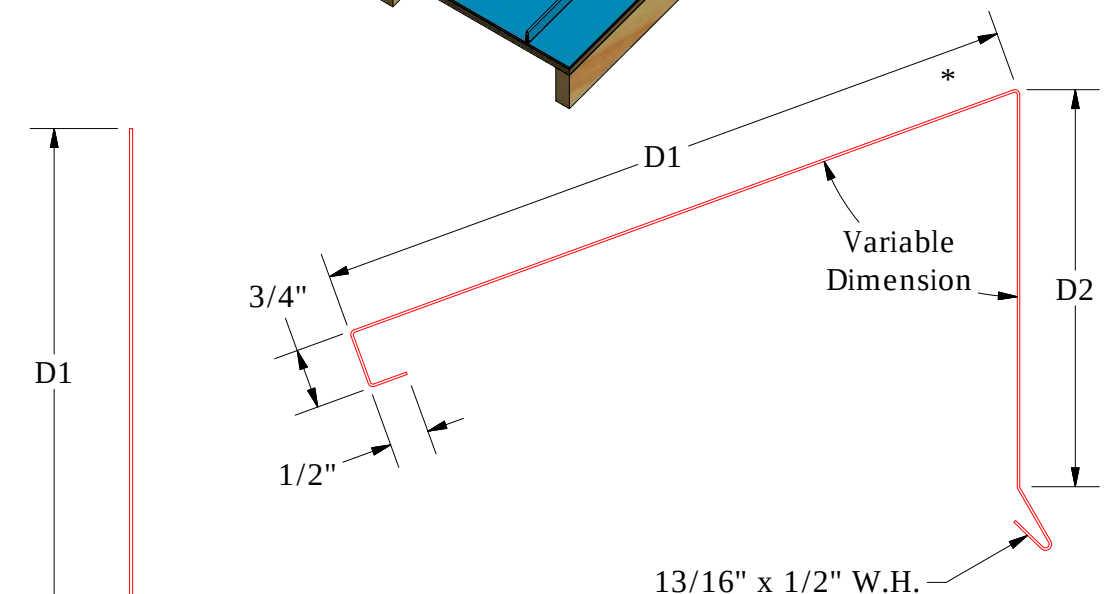
Vented Shed Ridge Cap PCA362-3:12 to 6:12 Slope D1=8 1/4" / D2=4 15/16" PCA364-6:12 to 9:12 Slope D1=9 1/4" / D2=5 3/16" PCA366-9:12 to 12:12 Slope D1=10 1/4" / D2=5 7/16"
