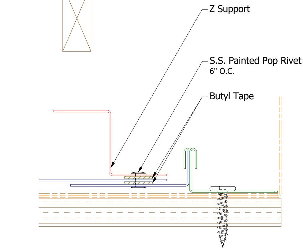
Butyl Tape Detail
