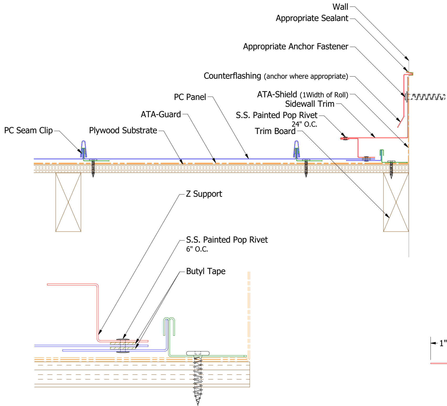
Butyl Tape Detail
