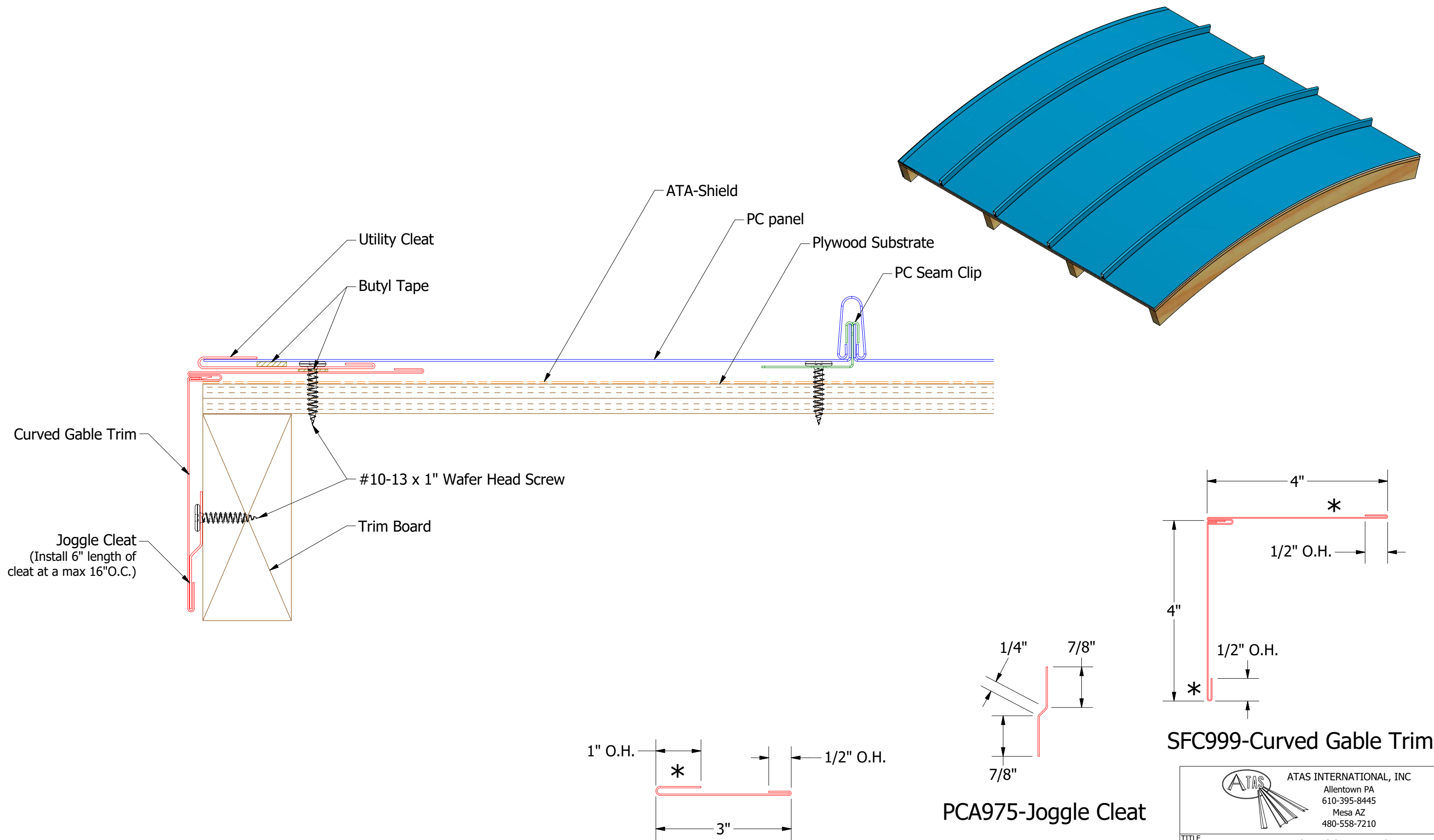
PCA962-Utility Cleat
