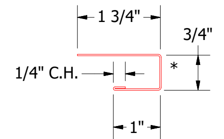
BGA034-J Channel
