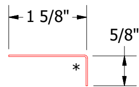
BGA680-Angle Trim
