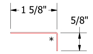
OPA680-Angle Trim
